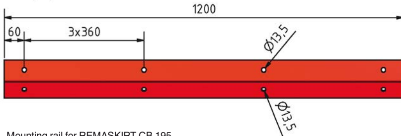
Mounting rail for REMASKIRT CB 195
