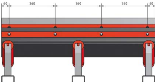
Mounting rail for REMASKIRT CB 195
